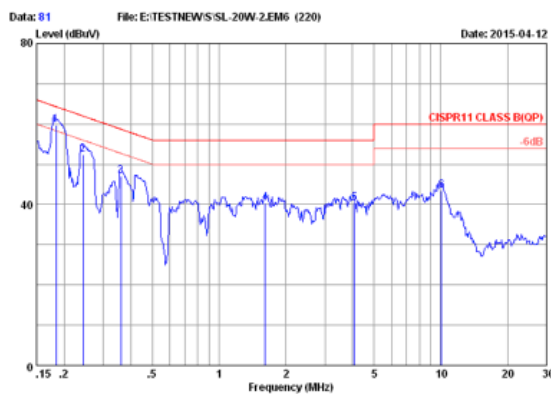
CISPR22 CLASS B QP 230V/50Hz 100% LOAD MARGIN: >4 dB
