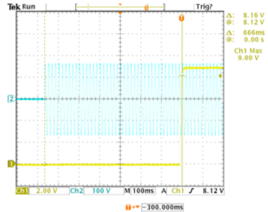
9V Turn-on delay, 115VAC
