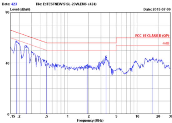
FCC15 CLASS B QP 100V/60Hz 100% LOAD MARGIN: >9 dB
