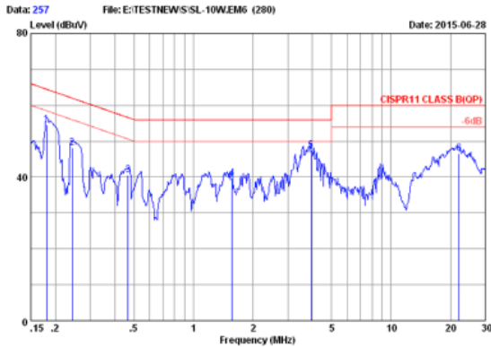
CISPR22 CLASS B QP 230V/50Hz 100% LOAD MARGIN: >8 dB
