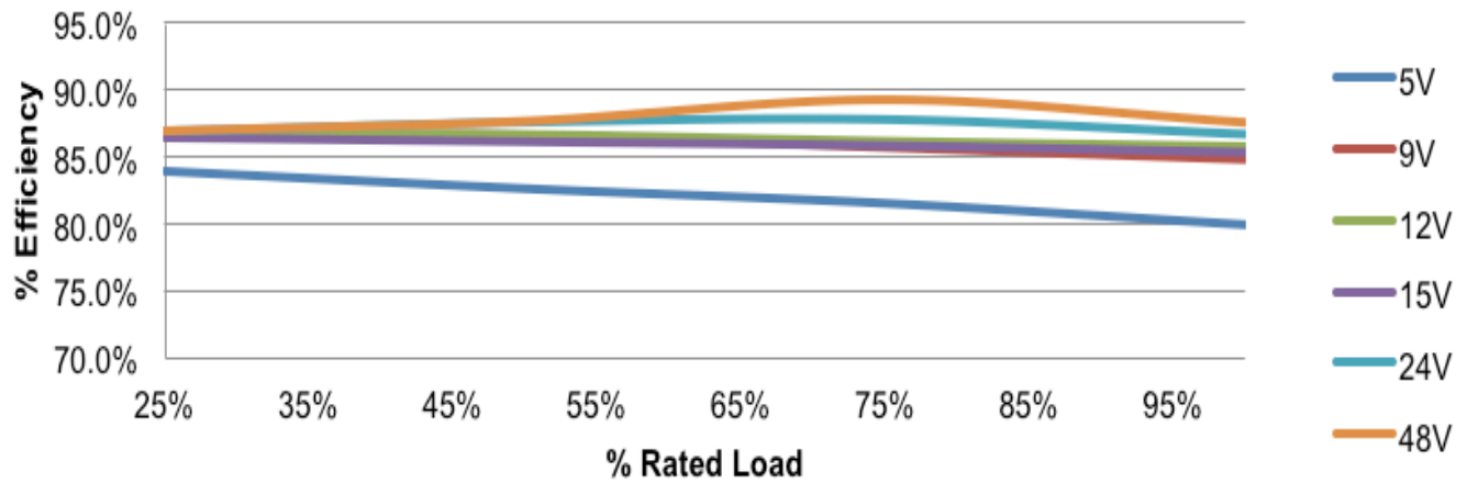
FIGURE 5b: ME20 Series Efficiency @ 115VAC.
