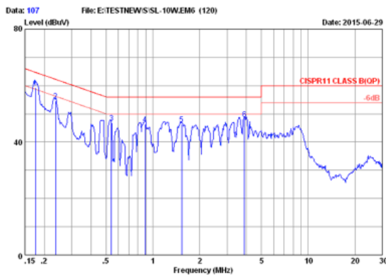
CISPR22 CLASS B QP 230V/50Hz 100% LOAD MARGIN: >5 dB
