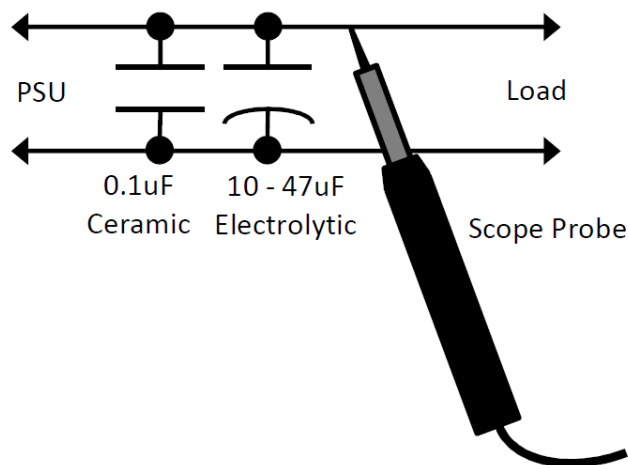
FIGURE 1: Noise measurement caps and probe with picture of the technique.
