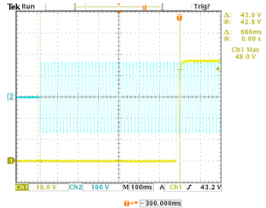
15V Turn-on delay, 115VAC
