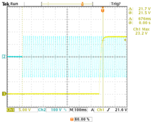
12V Turn-on delay, 115VAC
