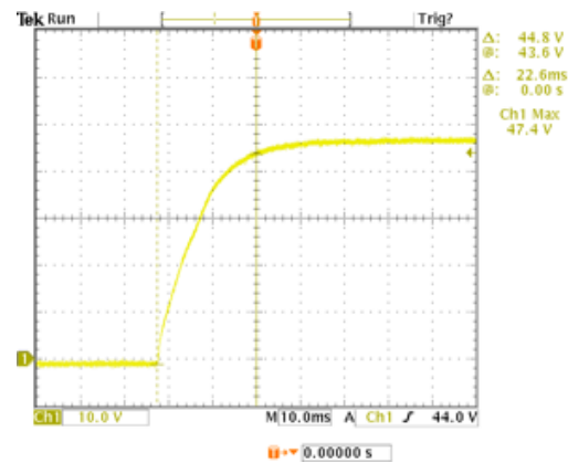
48V Rise Time
