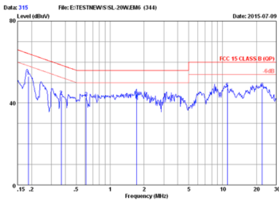
FCC15 CLASS B QP 100V/60Hz 100% LOAD MARGIN: >11 dB
