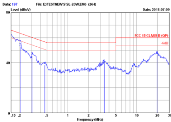
FCC15 CLASS B QP 100V/60Hz 100% LOAD MARGIN: >6 dB
