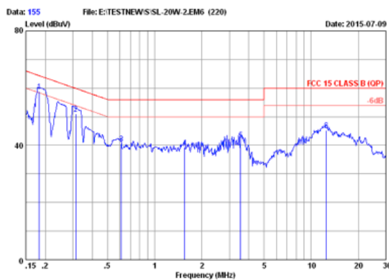
FCC15 CLASS B QP 100V/60Hz 100% LOAD MARGIN: >5 dB
