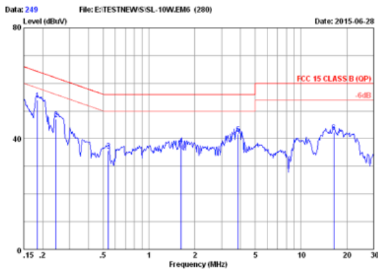
FCC15 CLASS B QP 100V/60Hz 100% LOAD MARGIN: >10 dB
