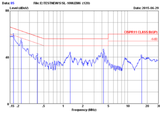
CISPR22 CLASS B QP 230V/50Hz 100% LOAD MARGIN: >6 dB
