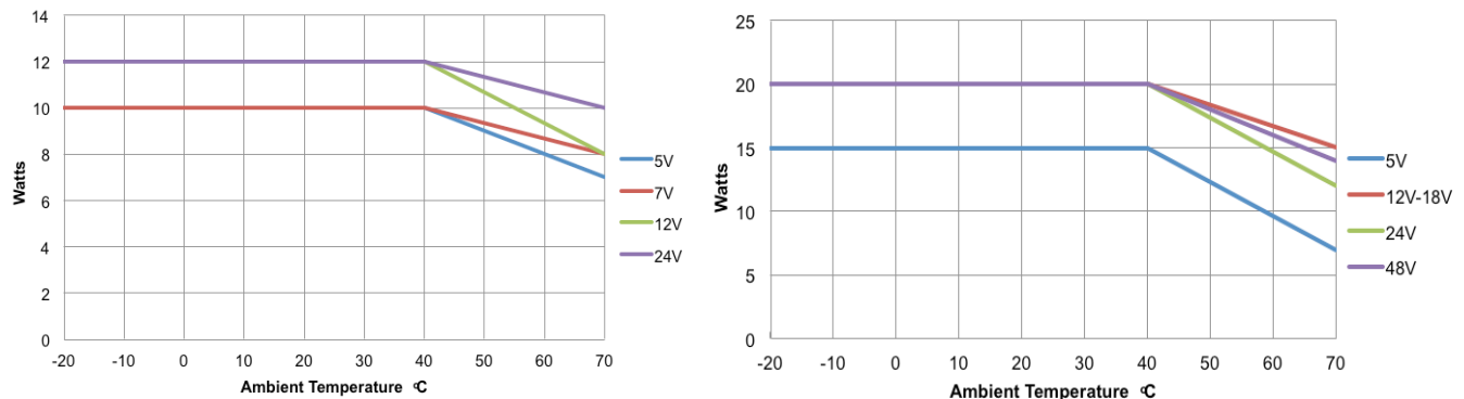
FIGURE 2: ME10 and ME20 family derating curve.
