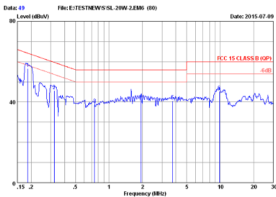
FCC15 CLASS B QP 100V/60Hz 100% LOAD MARGIN: >?? dB
