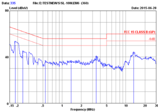
FCC15 CLASS B QP 100V/60Hz 100% LOAD MARGIN: >13 dB
