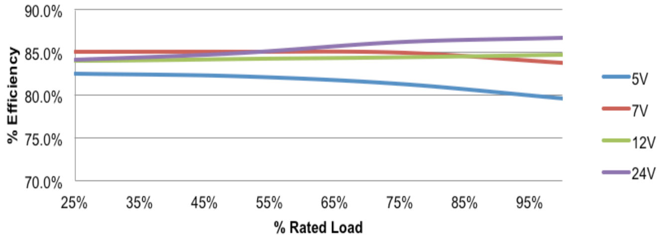
FIGURE 5a: ME10 Series Efficiency @ 115VAC.
