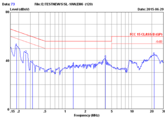
FCC15 CLASS B QP 100V/60Hz 100% LOAD MARGIN: >12 dB
