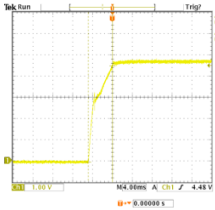
5V Rise Time
