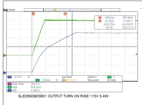
6W/9V Model Output Turn-On Rise Time
