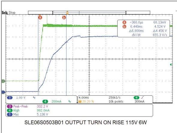
6W/5V Model Output Turn-On Rise Time
