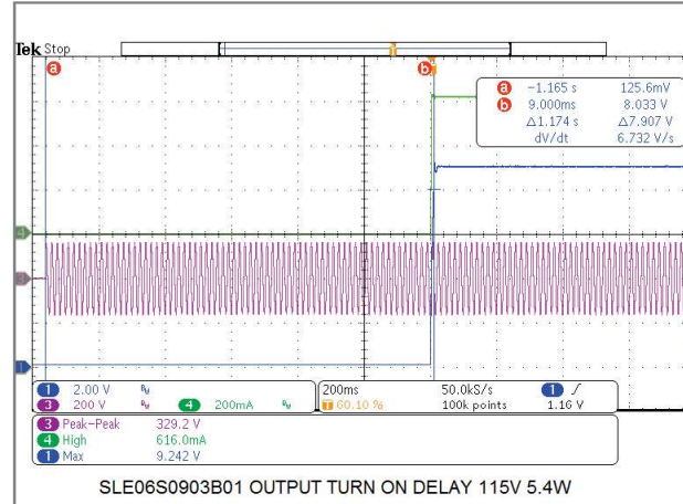
6W/9V Model Turn-On Delay Time
