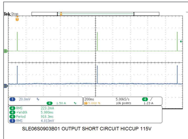
6W/9V Model Output Short Circuit Hiccup Mode
