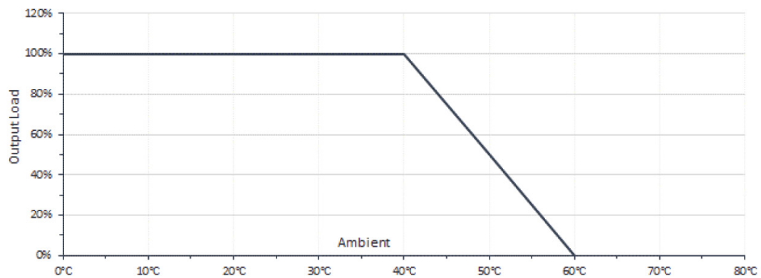
Figure 2: SLE06 family derating curve
