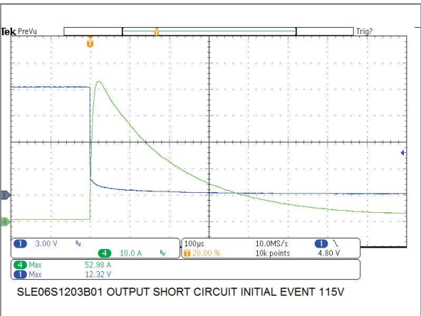
6W/12V Model Output Short Circuit Initial Event
