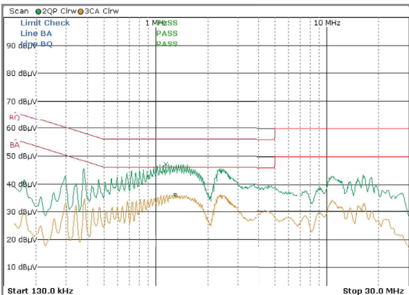
6W/9V Model _ Line 120V/60Hz 100% 9V@0.6A
