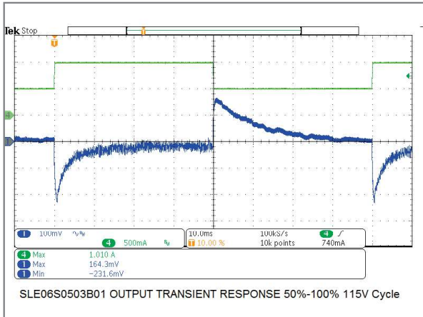
6W/5V Model Transient Response
