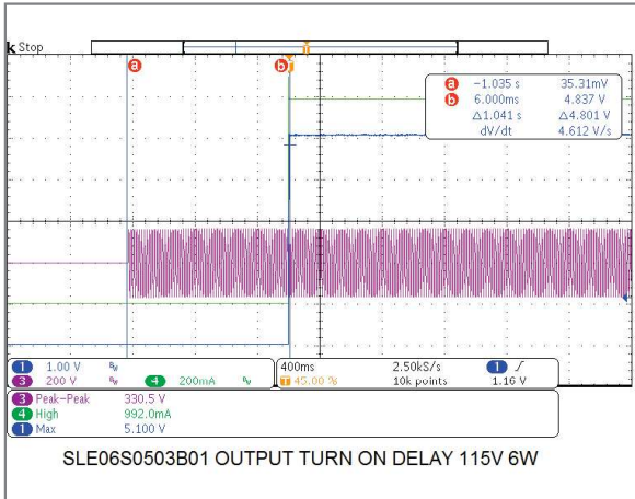
6W/5V Model Turn-On Delay Time
