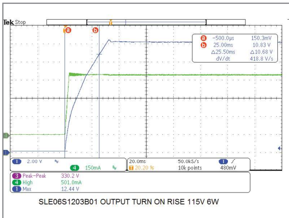
6W/12V Model Output Turn-On Rise Time
