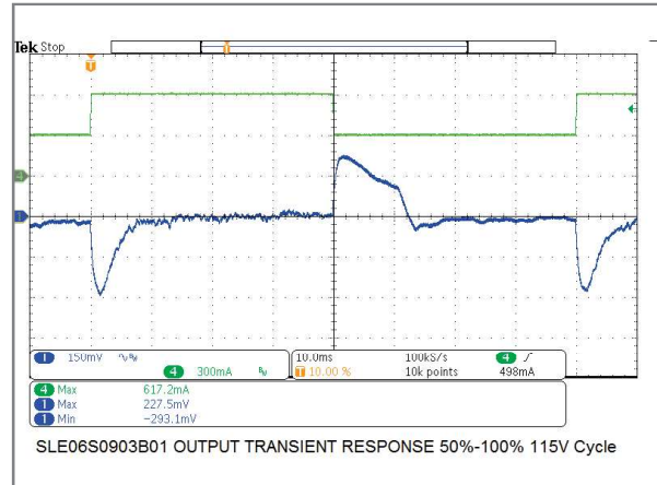
6W/9V Model Transient Response
