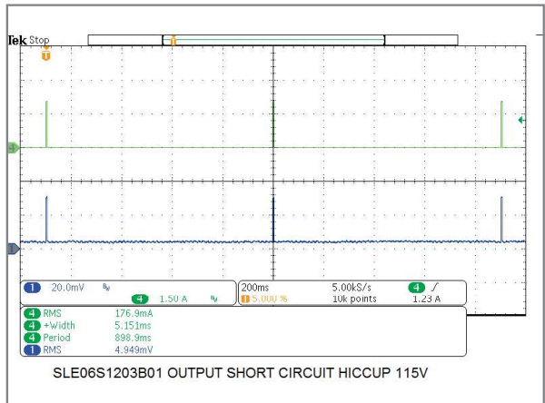
6W/12V Model Output Short Circuit Hiccup Mode
