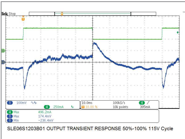
6W/12V Model Transient Response
