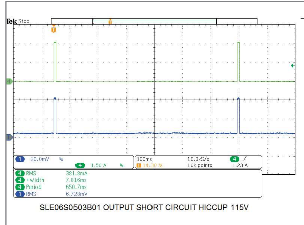
6W/5V Model Output Short Circuit Hiccup Mode
