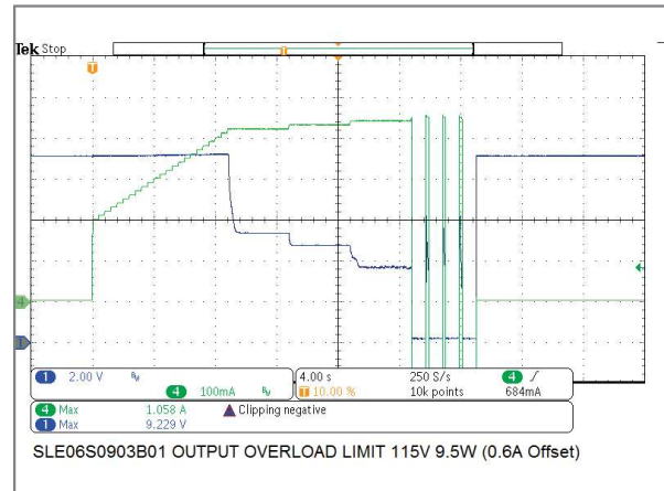
6W/9V Model Output Overload Protection
