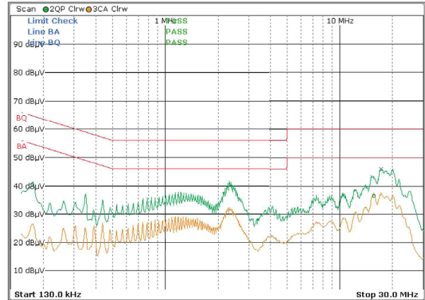
6W/5V Model _ Neutral 120V/60Hz 100% 5V@1.0A
