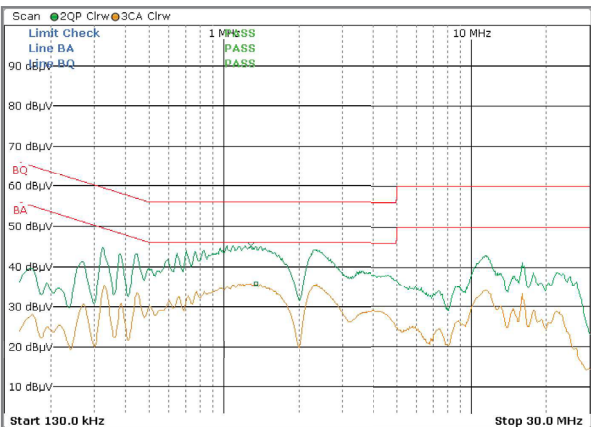
6W/12V Model _ Line 120V/60Hz 100% 12V@0.5A
