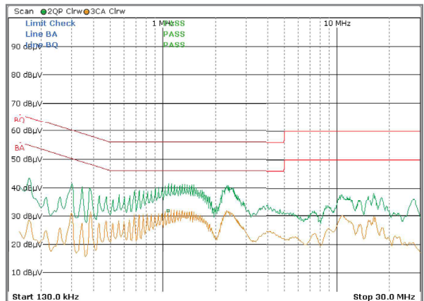
6W/9V Model _ Neutral 120V/60Hz 100% 9V@0.6A
