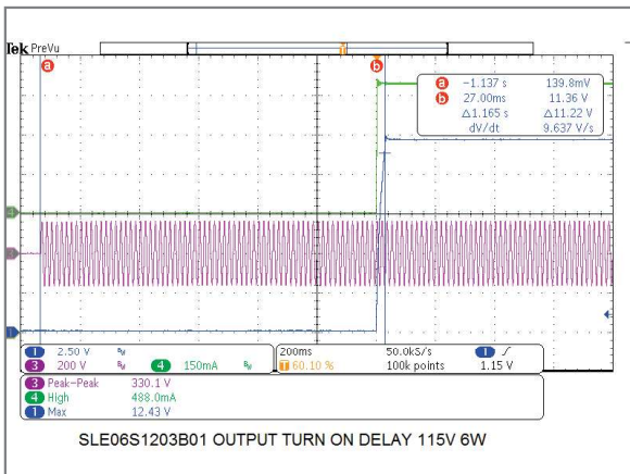
6W/12V Model Turn-On Delay Time
