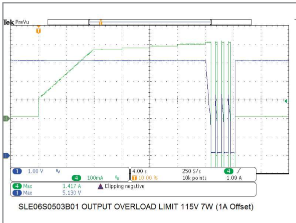
6W/5V Model Output Overload Protection
