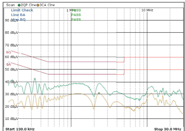
6W/12V Model _ Neutral 120V/60Hz 100% 12V@0.5A
