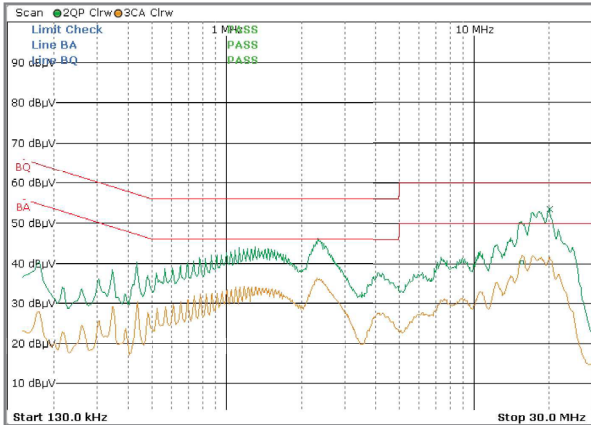
6W/5V Model _ Line 120V/60Hz 100% 5V@1.0A
