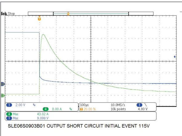
6W/9V Model Output Short Circuit Initial Event
