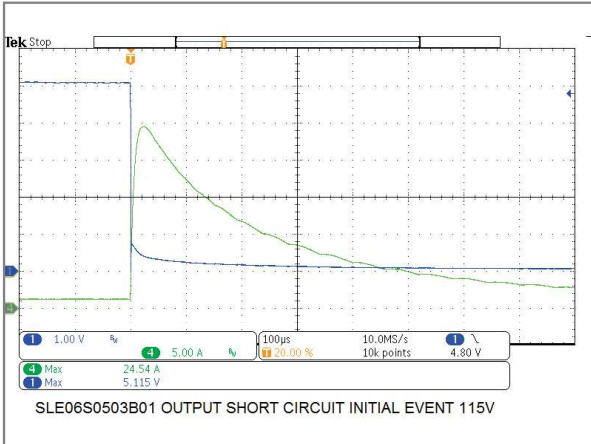
6W/5V Model Output Short Circuit Initial Event
