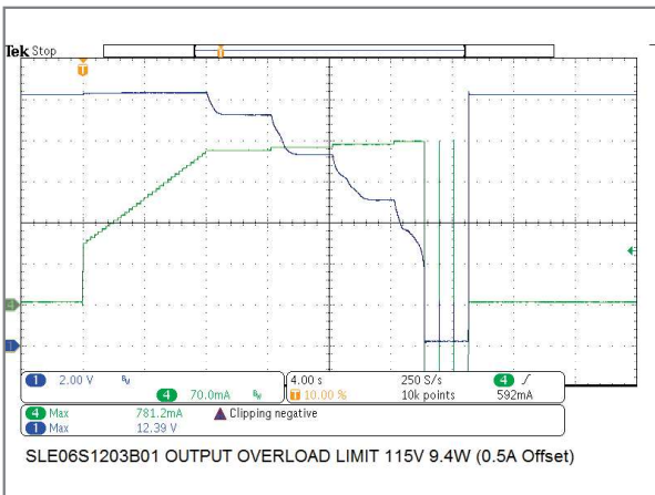
6W/12V Model Output Overload Protection
